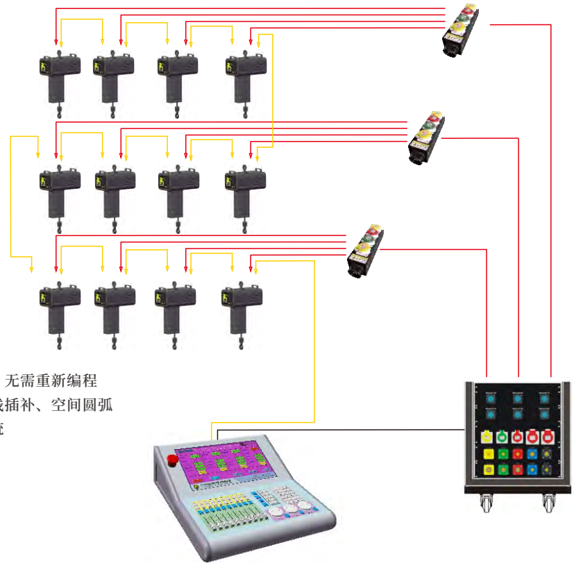
Intelligent CNC hoist system diagram
